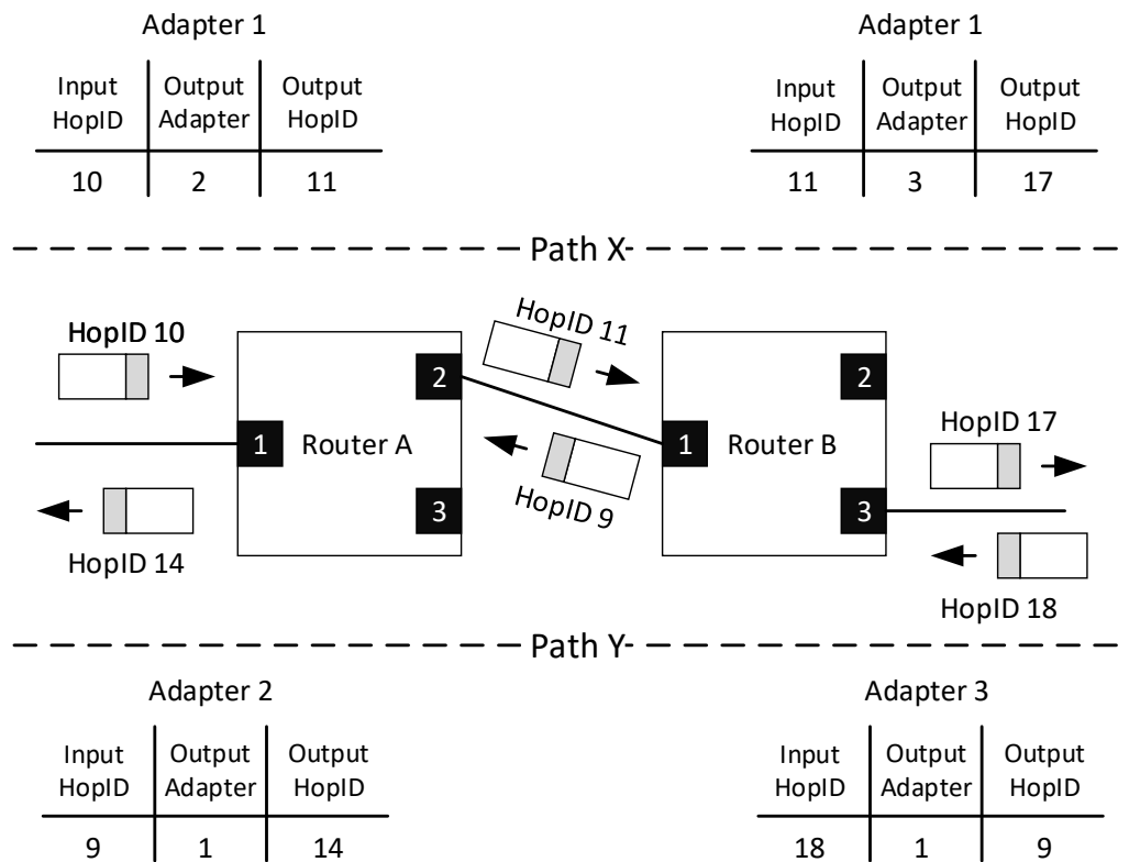
Figure 5-11. Routing Example
