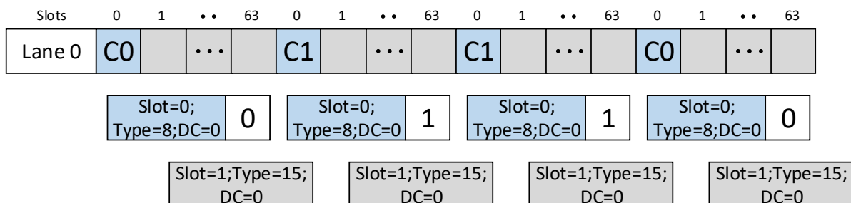
Figure 10-47. ACT Sequence, 1-Lane
