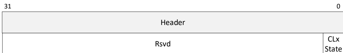
Figure 5-3. PM Packet for CL1 and CL2 States
