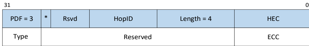
Figure 10-11. ACK Packet Format
