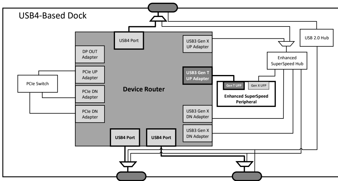
Figure 2-22. Example of a USB4-Based Dock with USB3 Gen T Tunneling Highlighted
