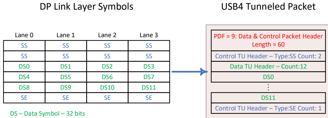
Figure 10-56 128b/132b MSA Packet Encapsulation
