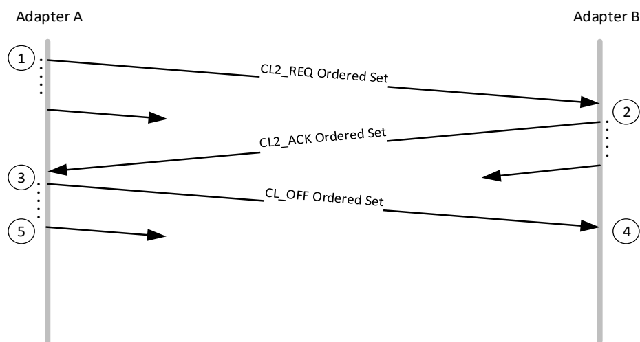
Figure C-1. Successful Entry to CL2 State
