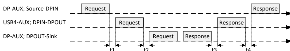
Figure 10-17. AUX Timing
