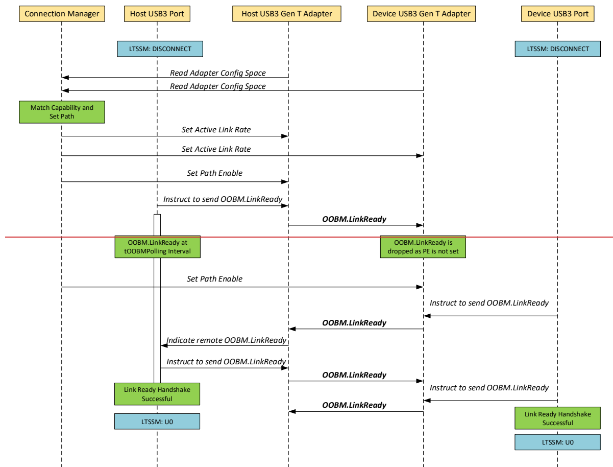
Figure 9-21. USB3 Gen T Link Ready Handshake Sequence
