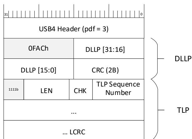
Figure 11-5. Encapsulation of 1 DLLP + 1 TLP into a Single Tunneled Packet
