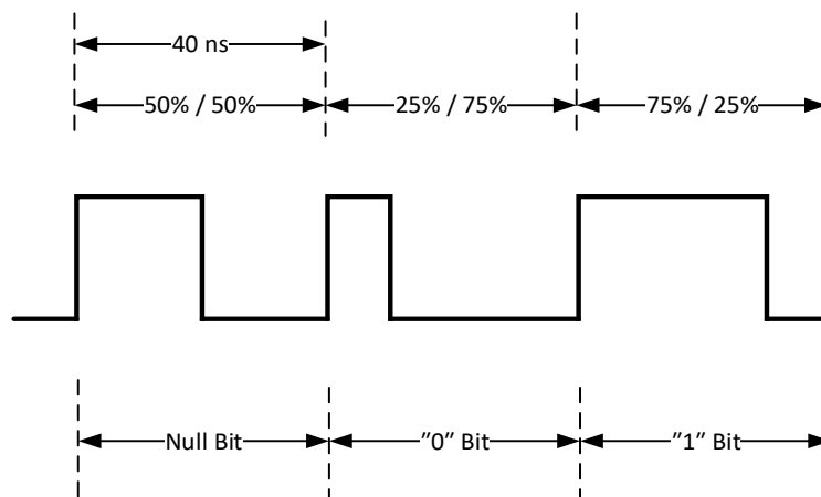
Figure D-1. Pulse Width Modulation
