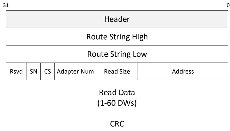
Figure 6-7. Read Response
