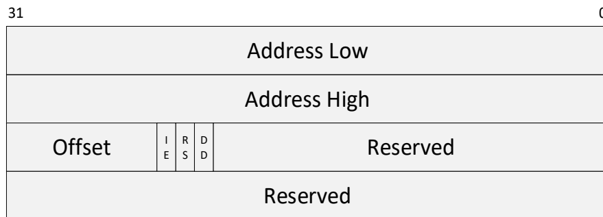
Figure 12-5. Receive Descriptor Structure (Posted by Host)
