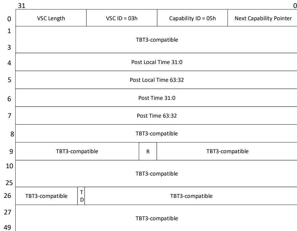
Figure 13-5. Structure of the Vendor Specific 3 Capability
