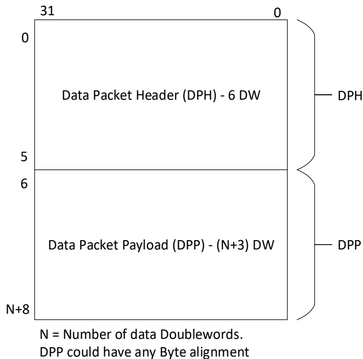
Figure 9-7. Structure of an Unsegmented USB3 Data Packet (Gen X)
