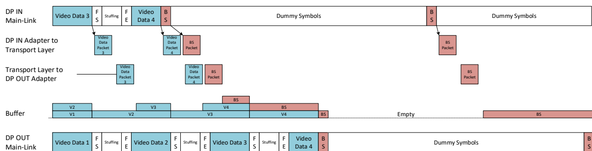
Figure 10-62. Active Video to Blanking for 8b/10b DP SST Link
