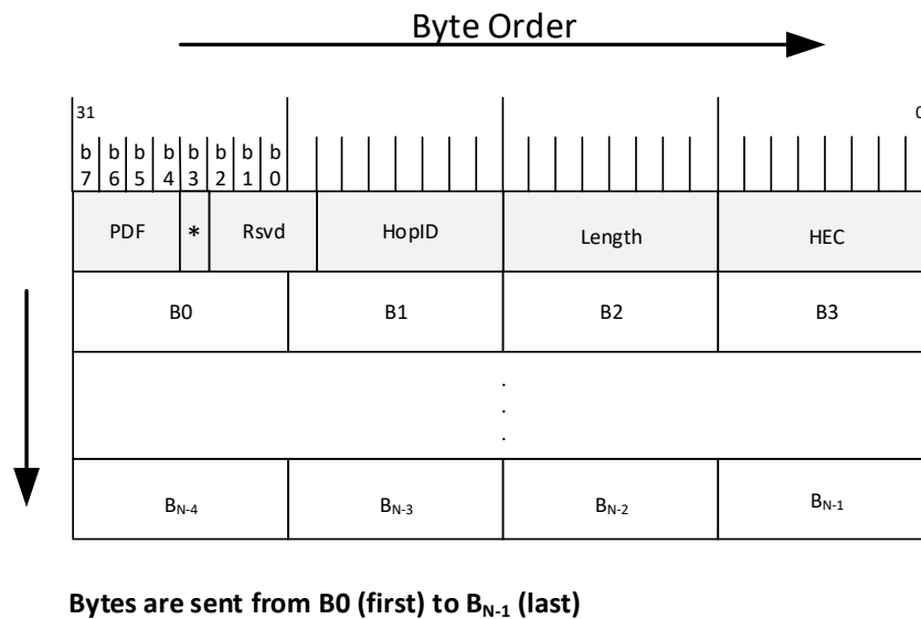
Figure 4-20. Byte Ordering of Transport Layer Packets to the Logical Layer
