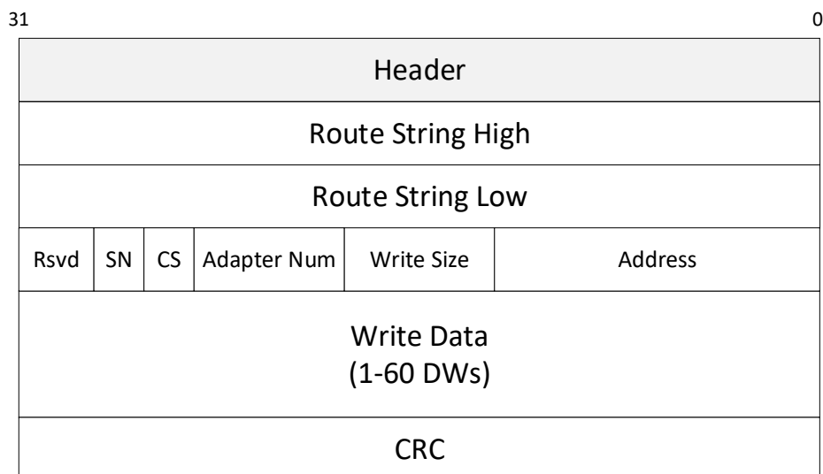
Figure 6-8. Write Request
