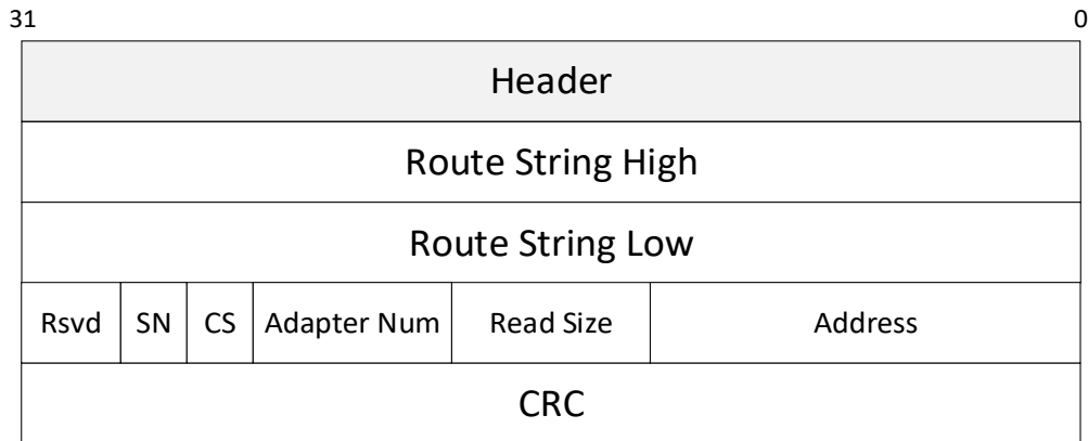
Figure 6-6. Read Request
