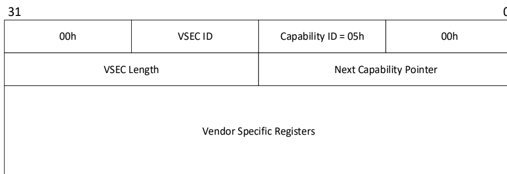
Figure 8-5. Structure of a Vendor Specific Extended Capability
