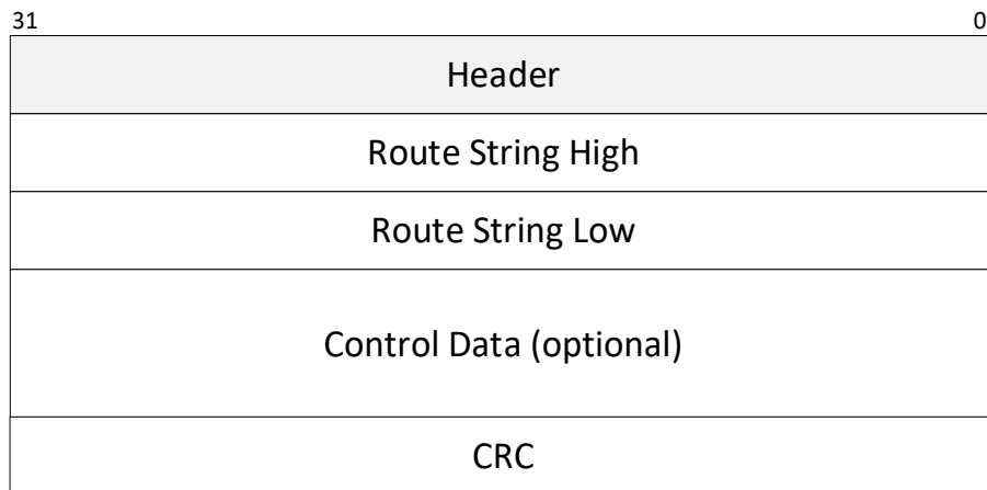
Figure 6-4 Control Packet Format
