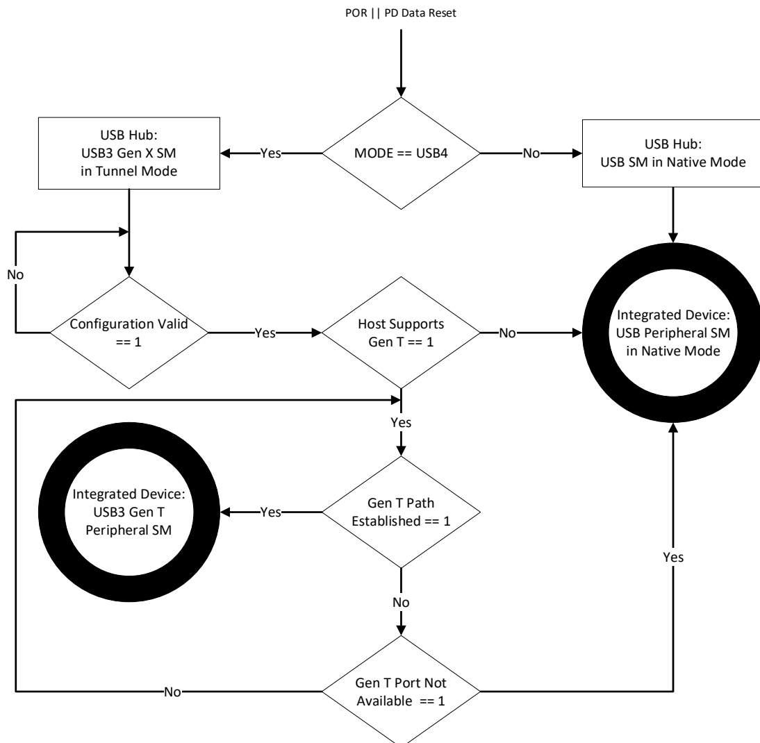
Figure 9-32. USB Compound Device Operational Device State Diagram
