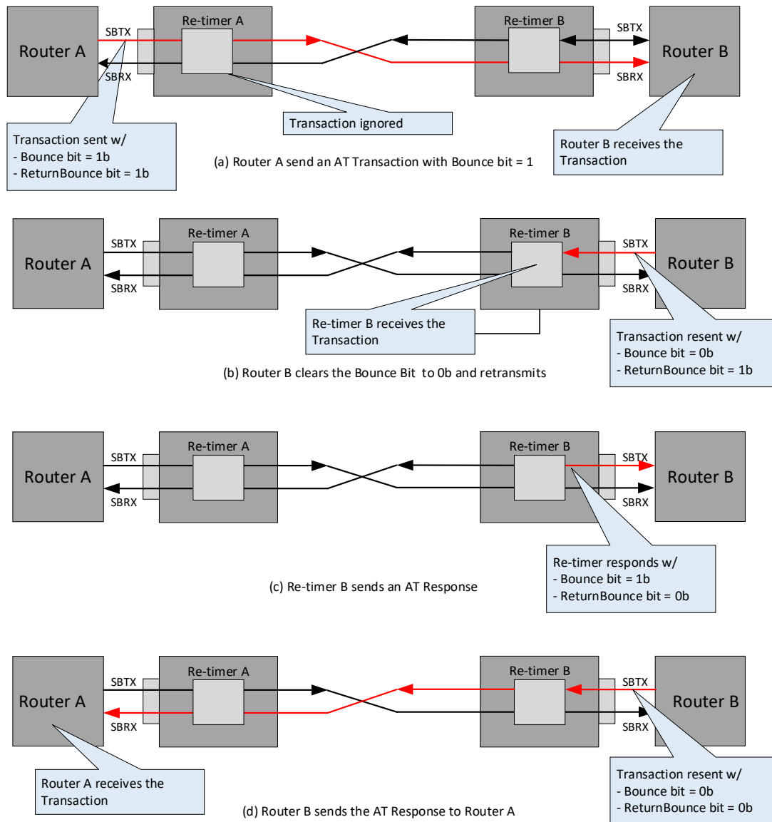
Figure 13-2. Bounce Mechanism
