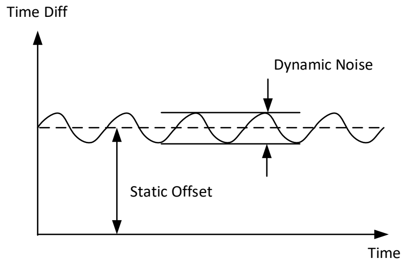
Figure 7-26. Dynamic Noise Types
