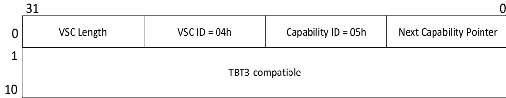
Figure 13-6. Structure of the Vendor Specific 4 Capability
