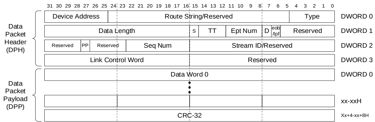
Figure 9-30. Data Packet
