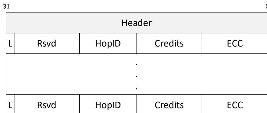
Figure 5-6. Credit Grant Packet Format
