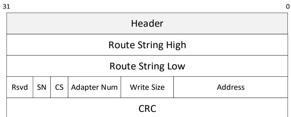
Figure 6-9. Write Response
