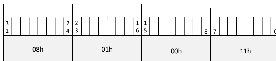
Figure 5-5. Idle Packet Contents
