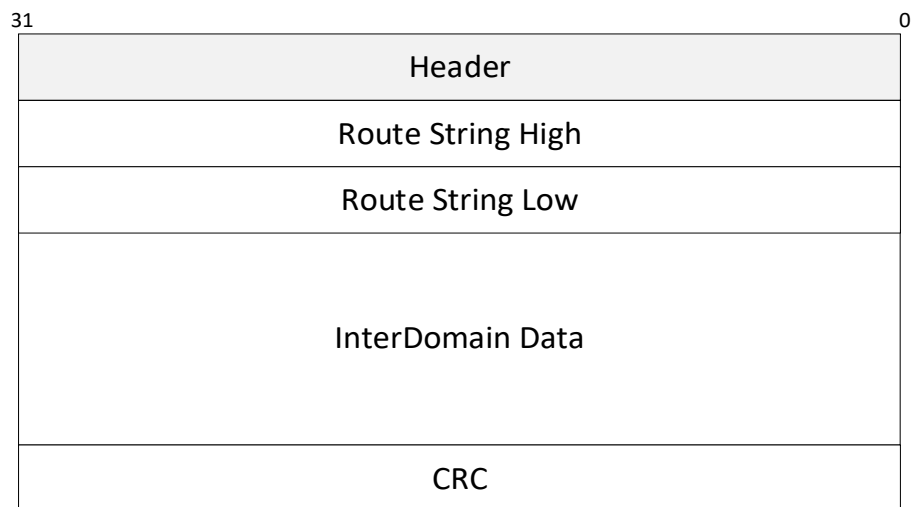
Figure 6-14. Inter-Domain Request
