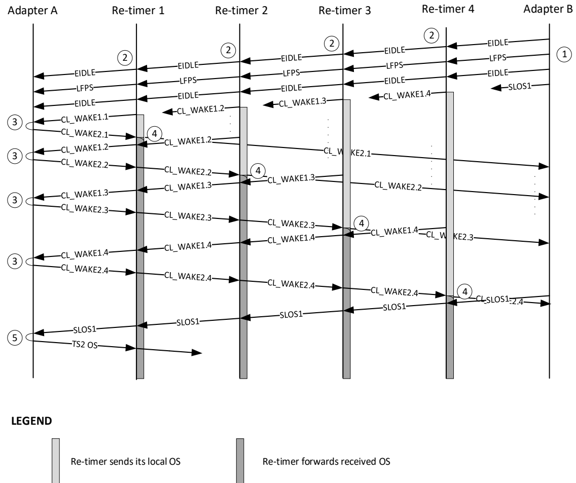
Figure C-10. CL0s Exit
