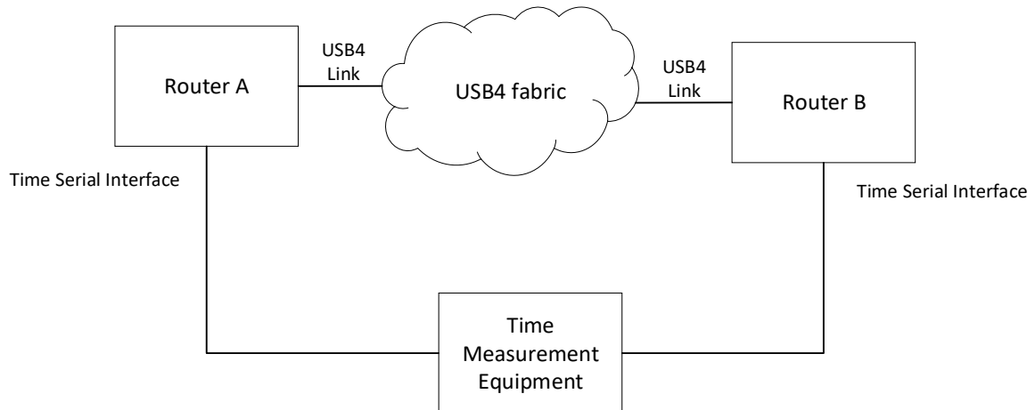
Figure 7-29. Measuring Method
